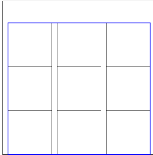
ypack => 'bottom'
