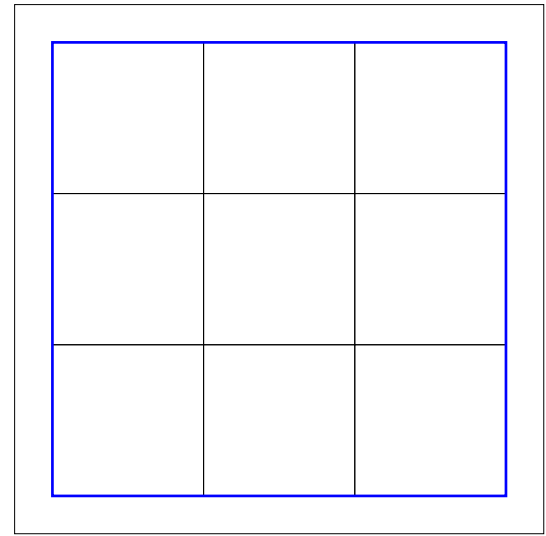
center => 1
